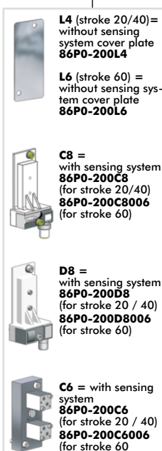
Inductive sensing system
