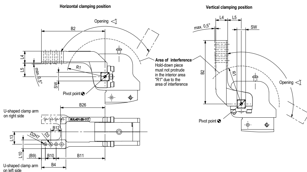
U-type left clamping position: horizontal
